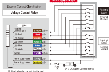
Lighting/Flashing/Alarm 24V DC
