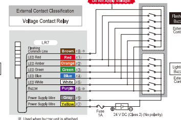
Lighting/Flashing/Alarm 24V DC
