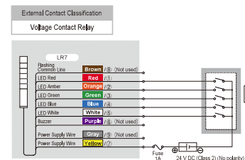
Lighting 24V DC
